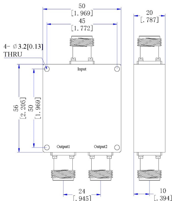
Dimensions (Unit: mm/[inch], Tolerance: ±0.3mm)
