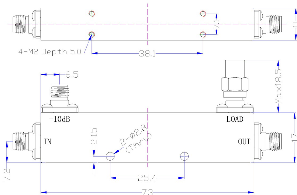
Dimensions (Unit: mm/[inch], Tolerance: ±0.5mm)
